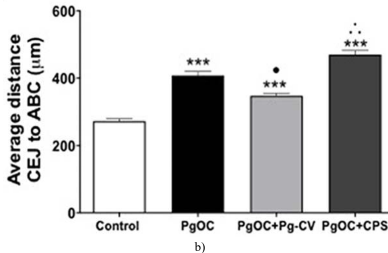
Figure 3. Vaccination with Pg-CV mitigates bone loss caused by oral P. gingivalis infection. (a) Example images of maxillae from four groups: untreated controls, mice challenged orally with P. gingivalis alone (Pg OC), mice challenged and immunized with Pg-CV (PgOC + Pg-CV), and mice challenged and immunized with purified P. gingivalis CPS (PgOC + CPS). (b) Assessment of alveolar bone loss. The distance between the alveolar bone crest (ABC) and the cemento-enamel junction (CEJ) was measured at 14 anatomical landmarks per mouse (7 per hemimaxilla; n = 10 mice per group). Measurements were combined to calculate group means \pm SEM. Statistical comparisons were performed using ANOVA with Tukey's post hoc test: *** P < 0.001 versus Control, • P < 0.05 versus Pg OC (decrease), •• P < 0.05 versus Pg OC (increase).
