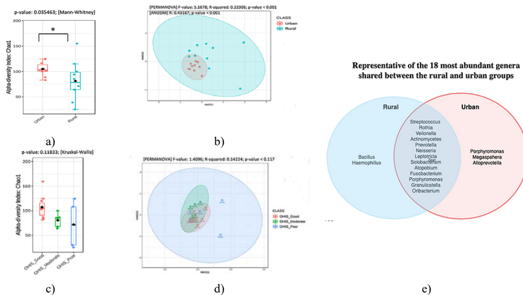
Figure 1. Overview of Oral Microbiota Diversity and Community Structure in Urban and Rural Populations.
