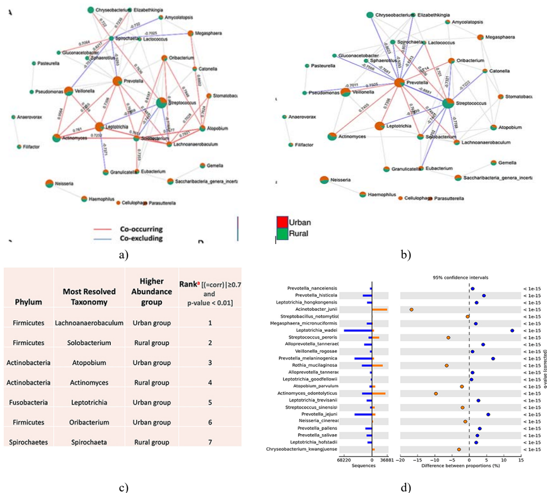
Figure 3. Co-occurrence Networks in the Oral Microbiome Across Populations
