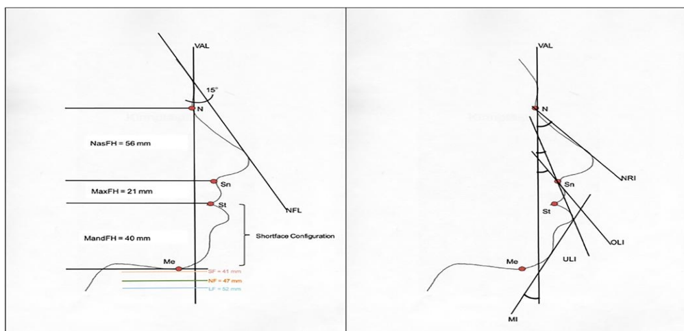
Figure 1. Schematic of Brons–Mulié measurements in vertical (left) and sagittal (right) planes. NFL nasofrontal line; VAL vertical reference line at 15°; NasFH nasofacial height; MaxFH maxillofacial height; MandFH mandibulofacial height; SF short-face limit; LF long-face limit; NF optimal mandibulofacial height;
